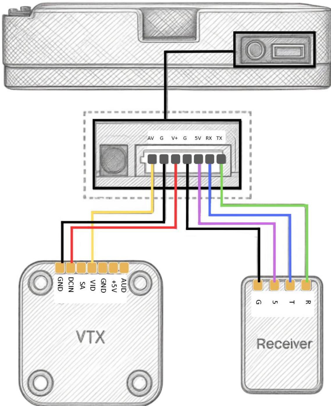
Fig.2. Schematic diagram of connection between ground end, VTX and receiver
