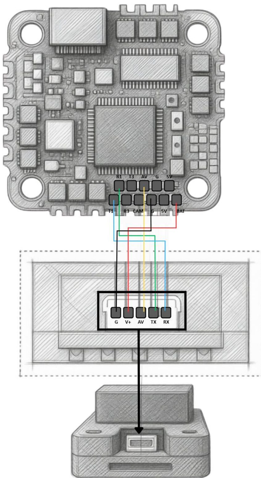
Fig.1. Schematic diagram of the connection between the sky end, the flight control transmission and receiver
