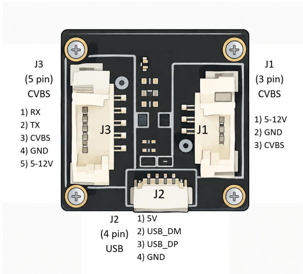
Fig.2. Wiring diagram
