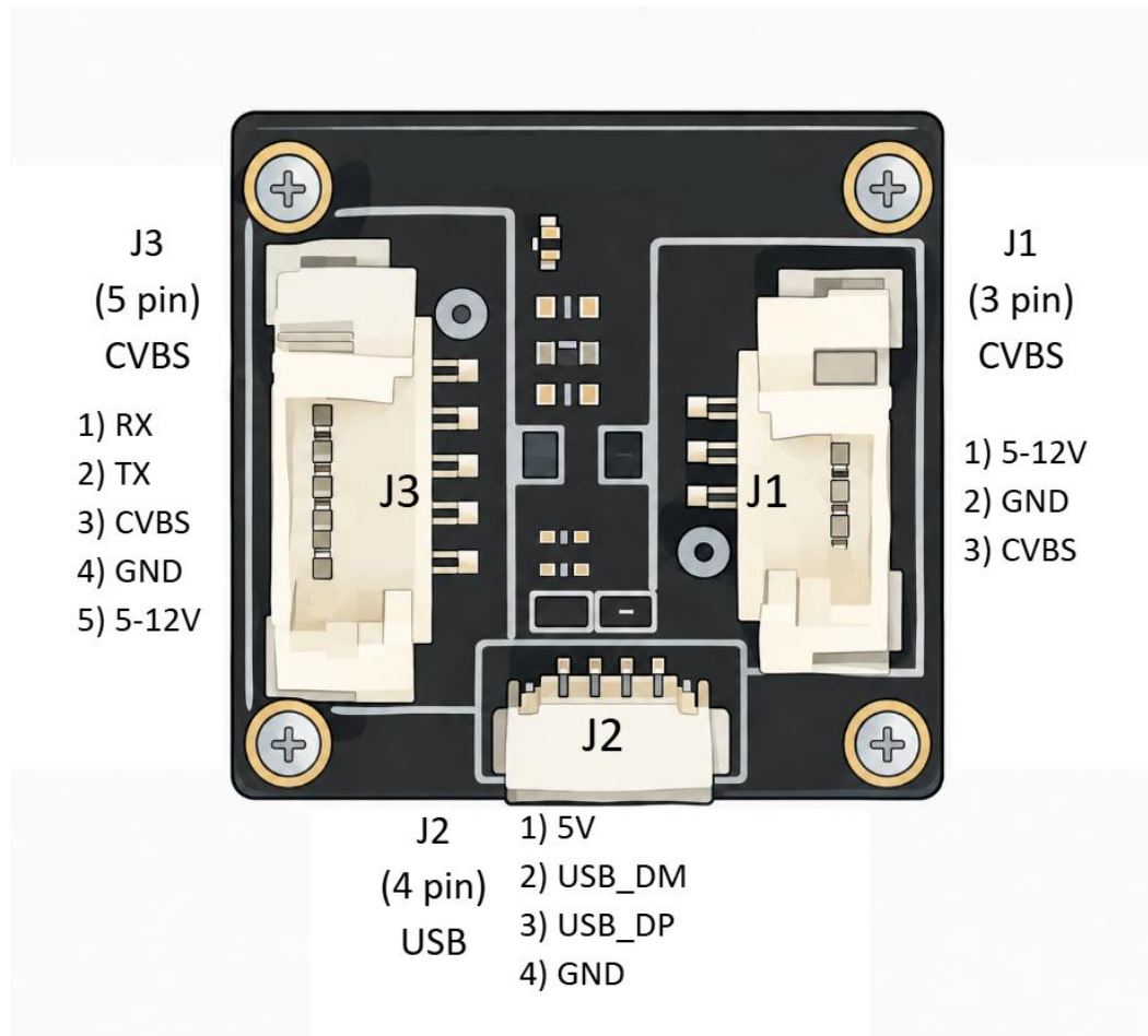
Fig.2. Wiring diagram
